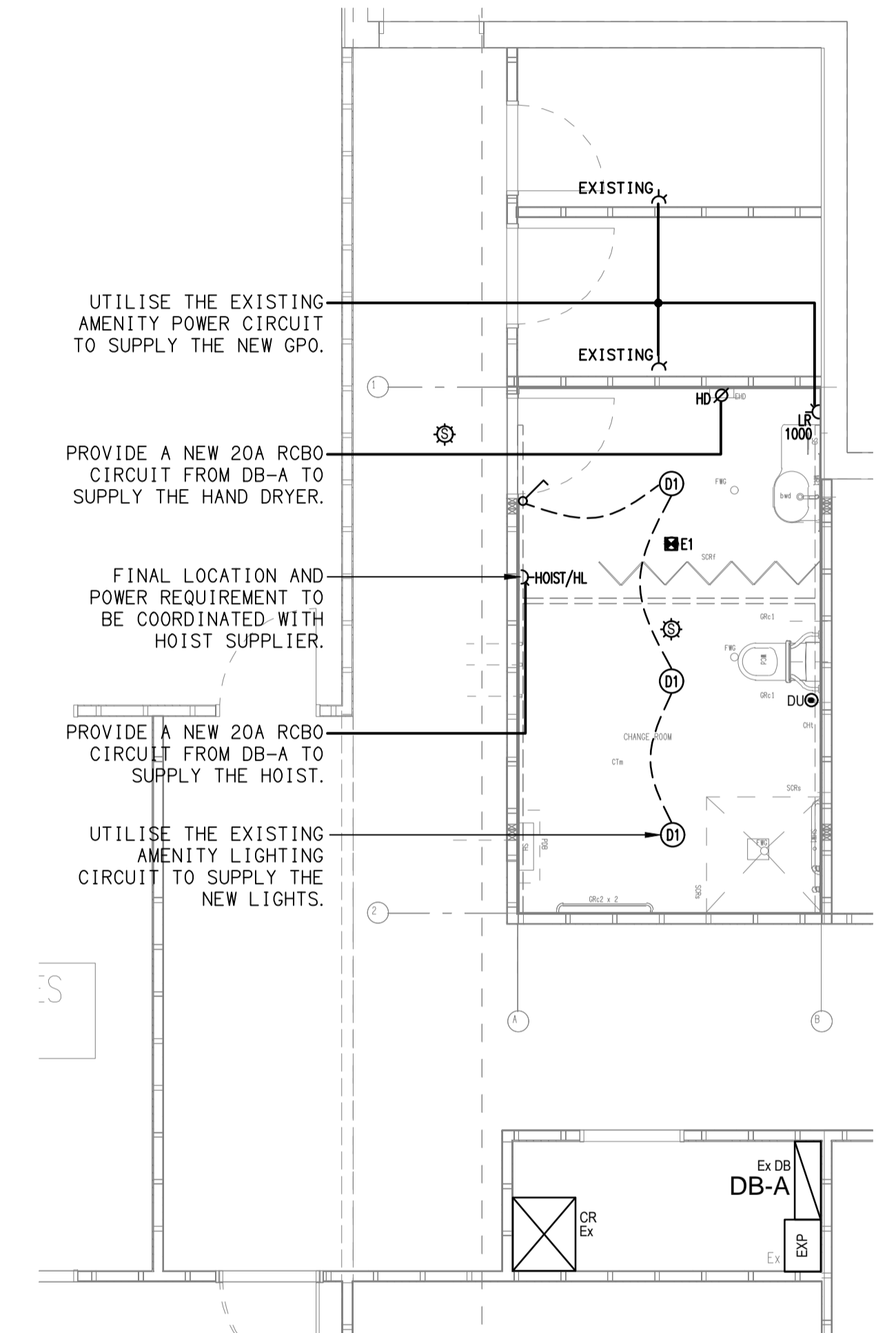
PART PLAN PROPOSED ELECTRICAL WORKS SCALE 1:50
